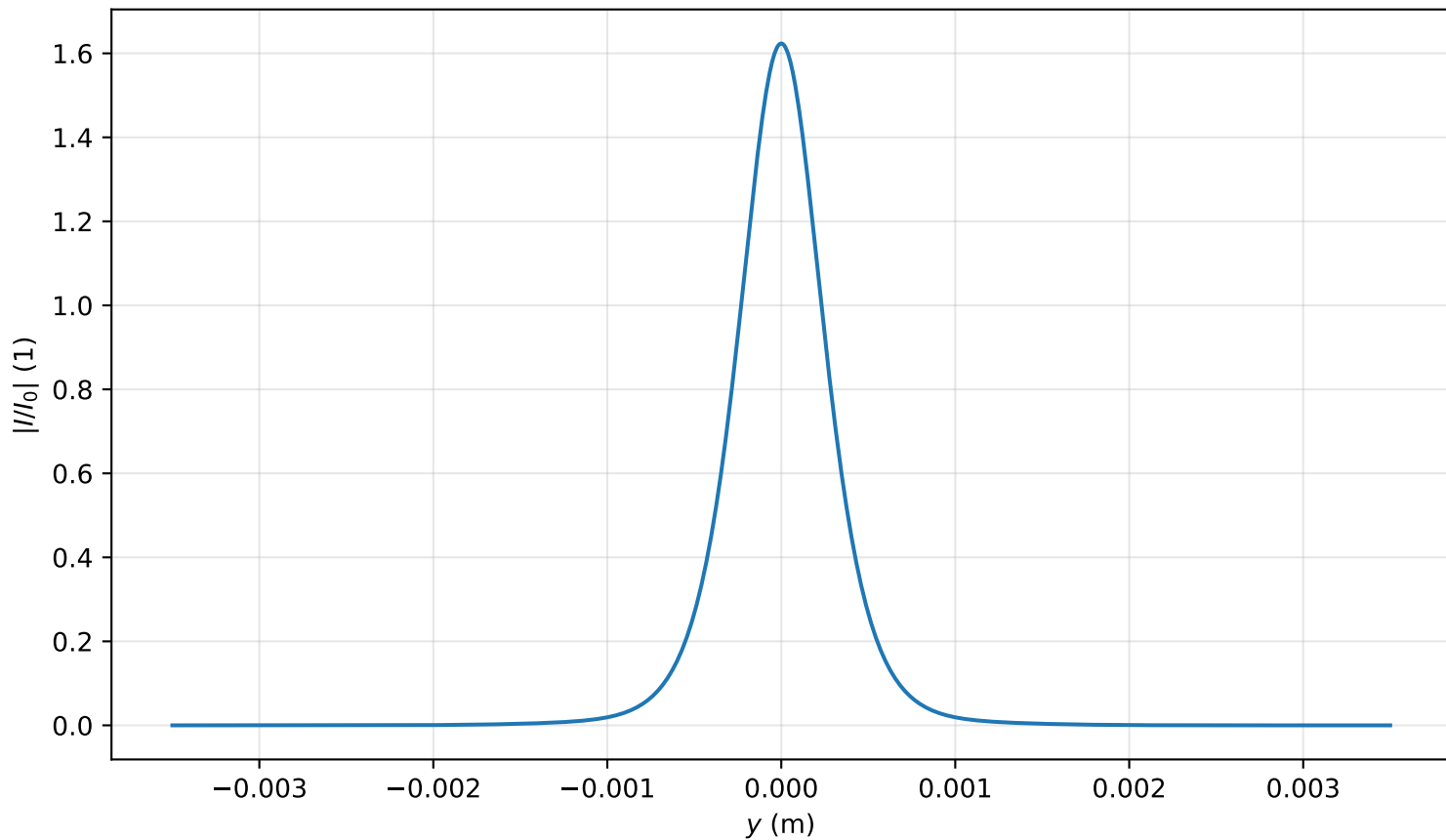
Intensity profile I(x = 0, y, z = 2.468)/I_0 , P_{in}=0.9P_{cr} , artificial time
